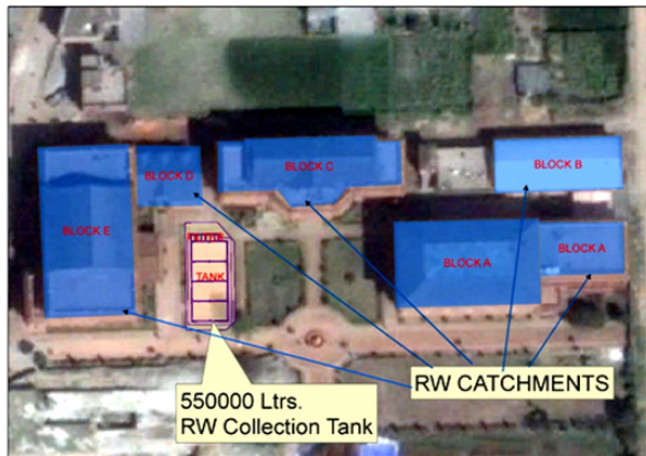
Figure 6: RWH in Khwopa Engineering College
