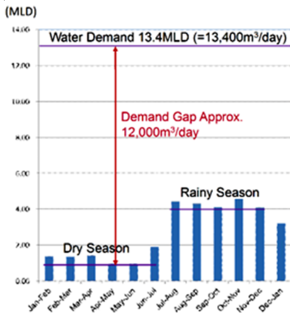
Figure 3: water Demand and Supply in Bhaktapur Municipality (HAZAMA ANDO CORPORATION and NJS CONSULTANTS Co., Ltd., 2015)
