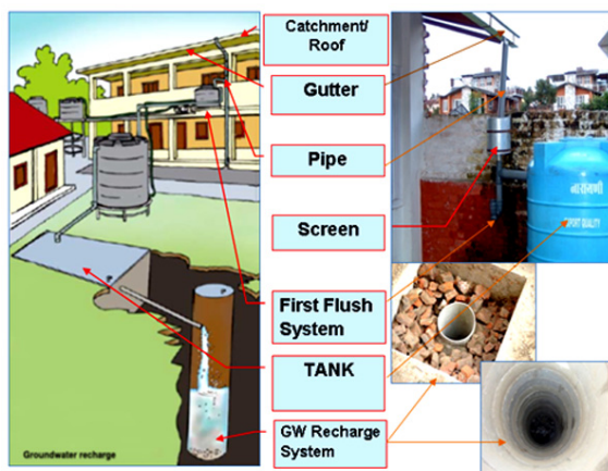
Figure 9: Rainwater Harvesting and Groundwater Recharge System
