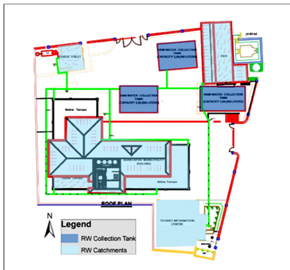
Figure 7: Proposed RWH plan in Bhaktapur Municipality Office
