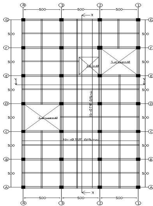
First Floor Slab reinforcement(Bottom bar)
