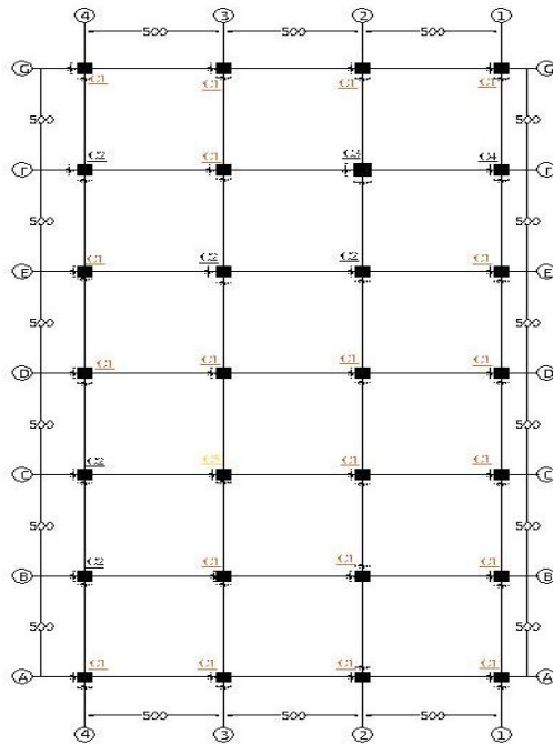
COLUMN LAYOUT PLAN
