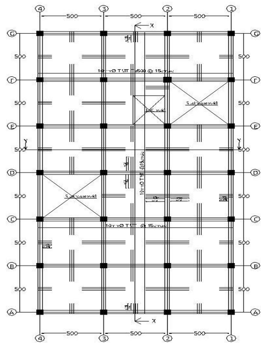
First Floor Slab reinforcement(Top bar)
